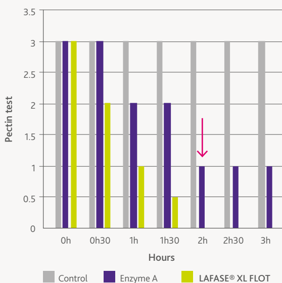
Depectinisation kinetics at 20°C (68°F)
